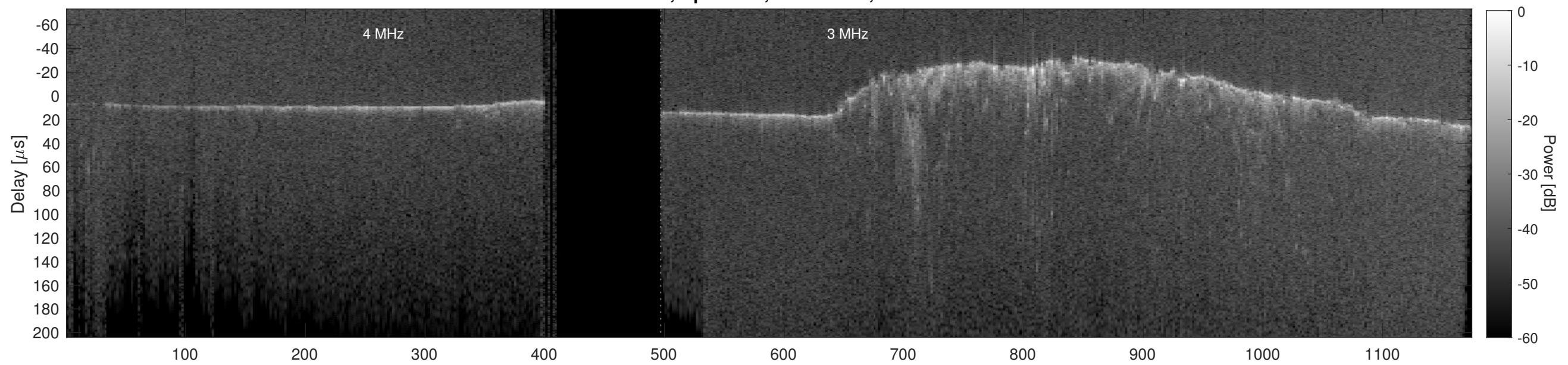
Orbit 15586, Cluttergram
