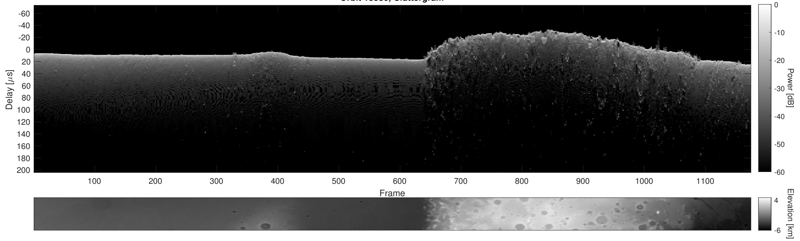
Orbit 15586, Cluttergram
