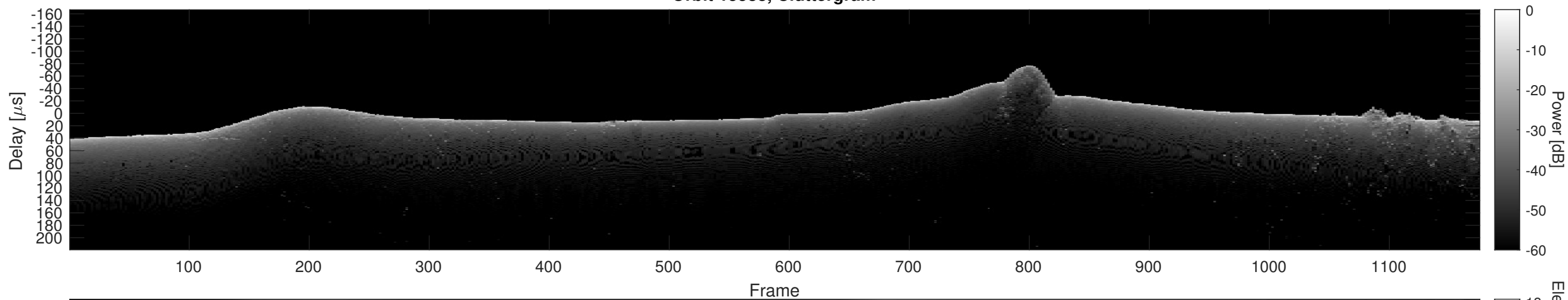
Orbit 15588, Cluttergram
