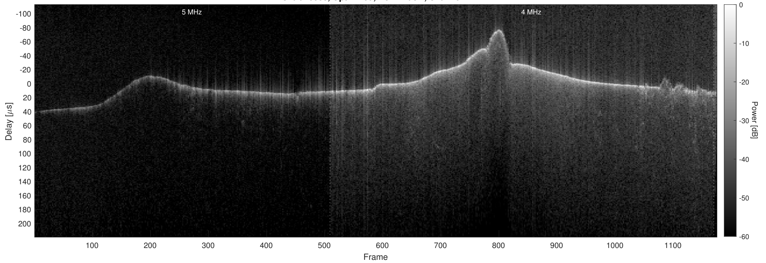
Orbit 15588, Optimized, No Window, Channel 2
