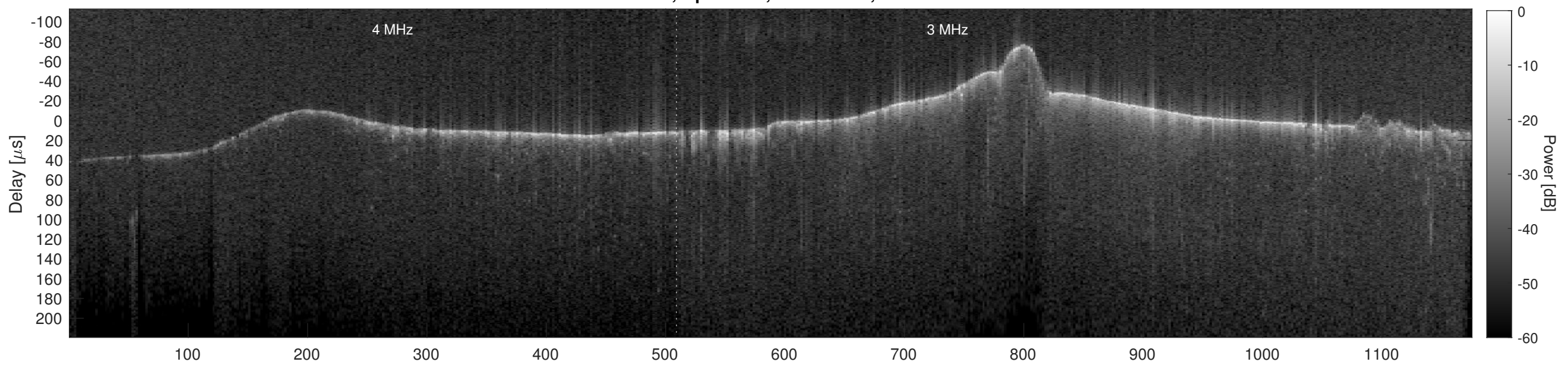
Orbit 15588, Cluttergram
