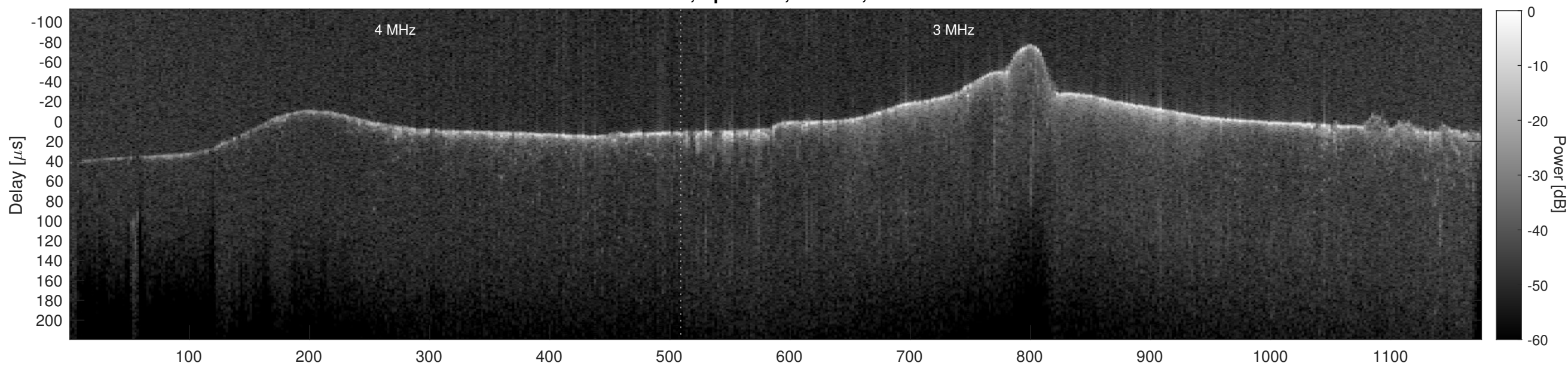
Orbit 15588, Cluttergram
