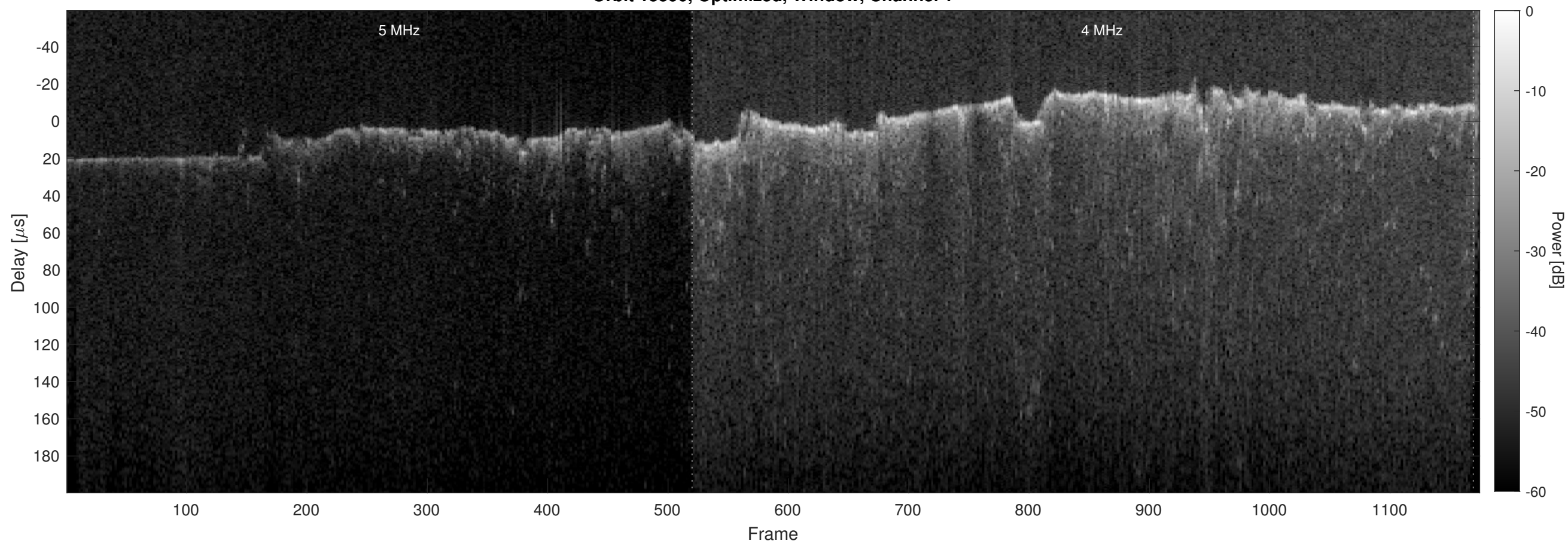
Orbit 15590, Optimized, Window, Channel 2
