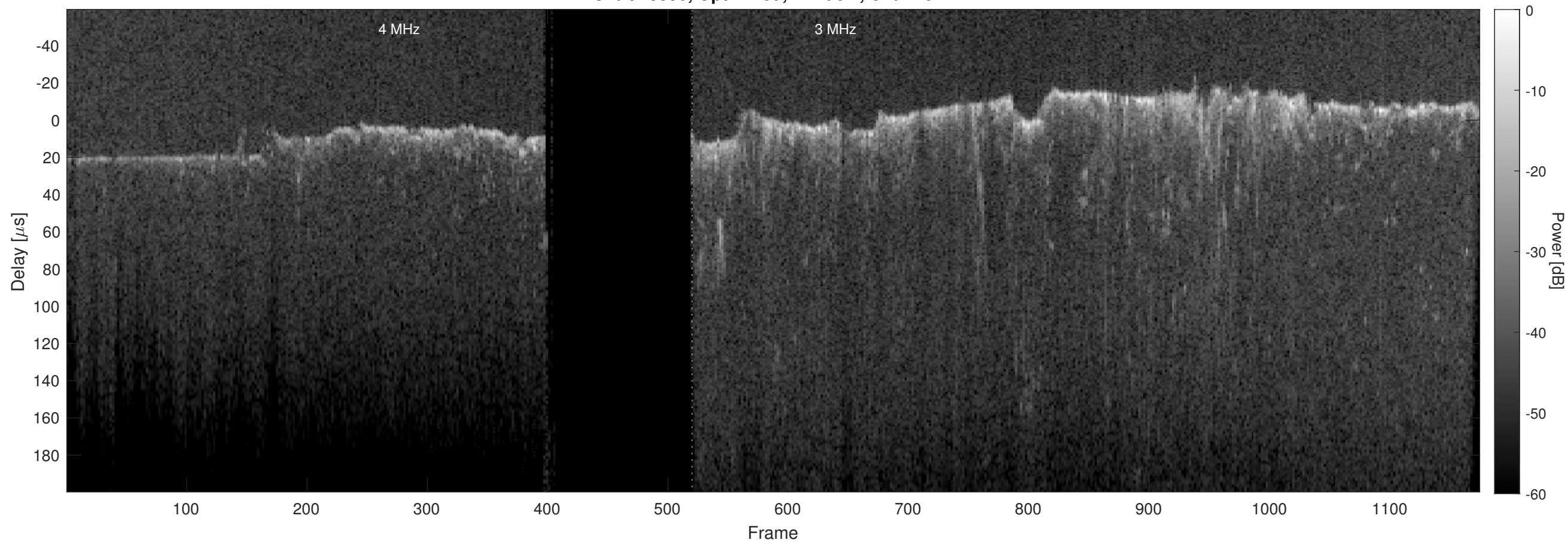
Orbit 15590, Optimized, Window, Channel 2
