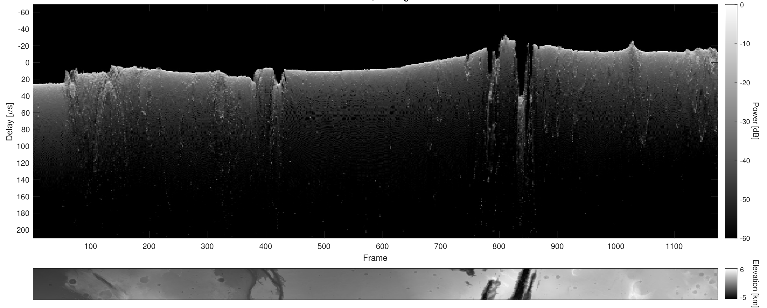
Orbit 15591, Cluttergram
