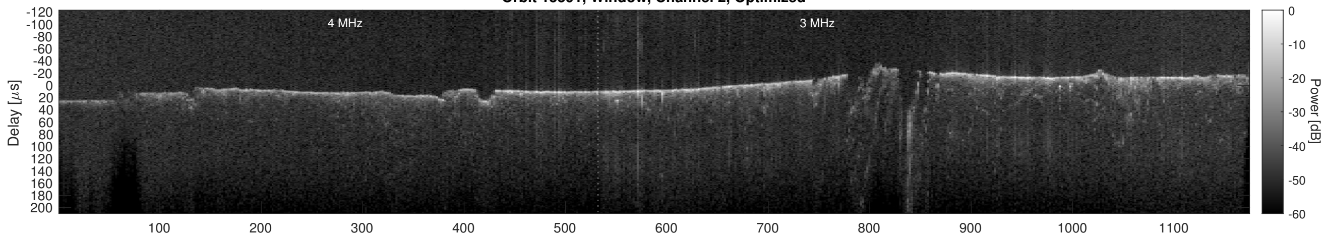
Orbit 15591, Cluttergram
