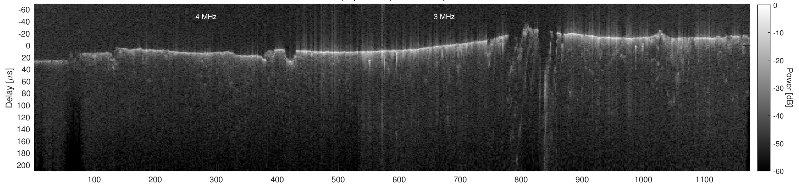
Orbit 15591, Cluttergram
