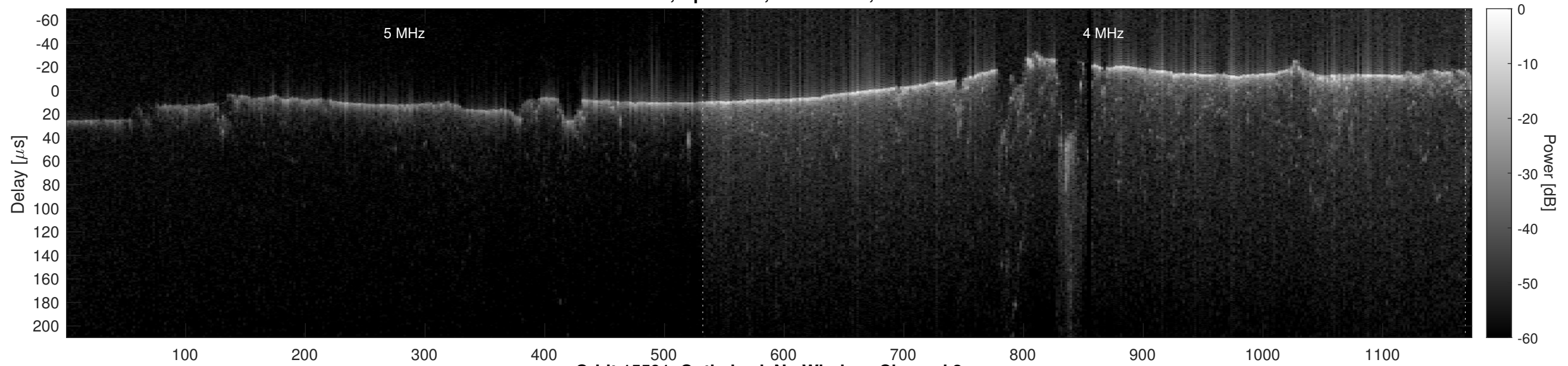
Orbit 15591, Optimized, No Window, Channel 2
