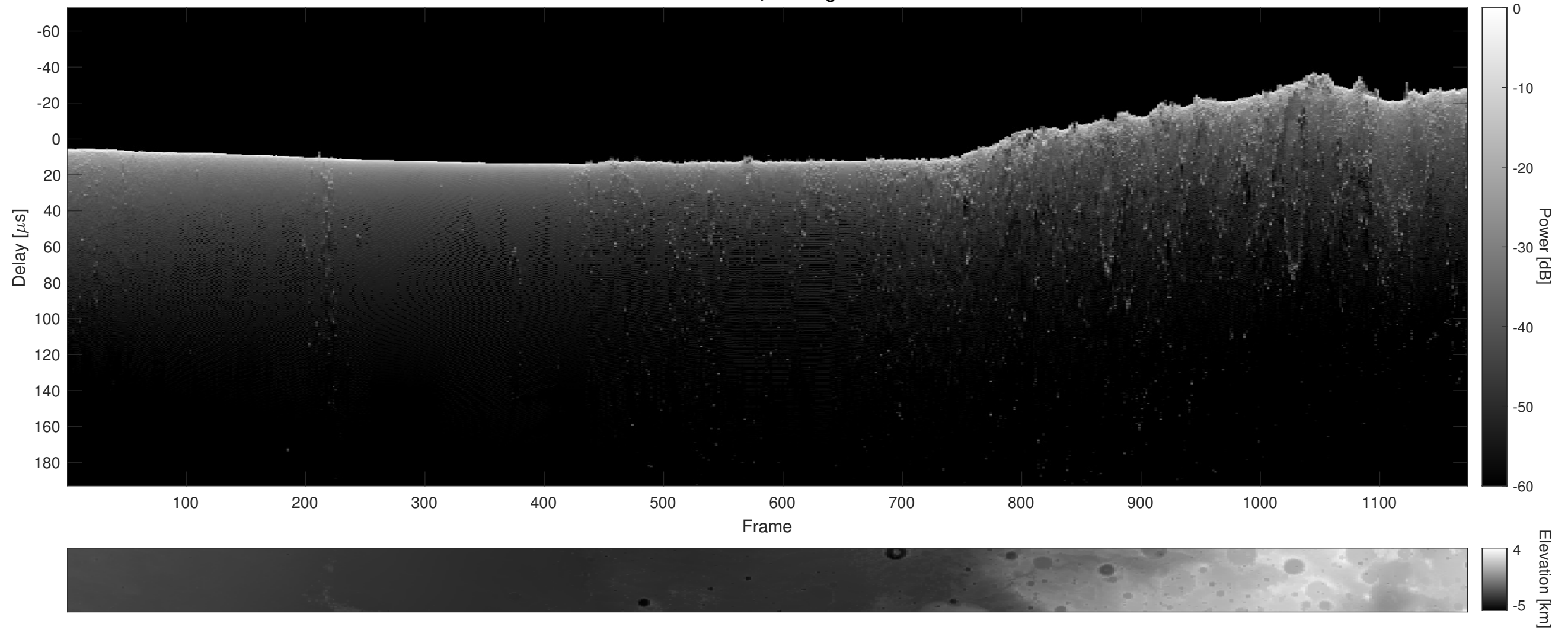
Orbit 15592, Cluttergram
