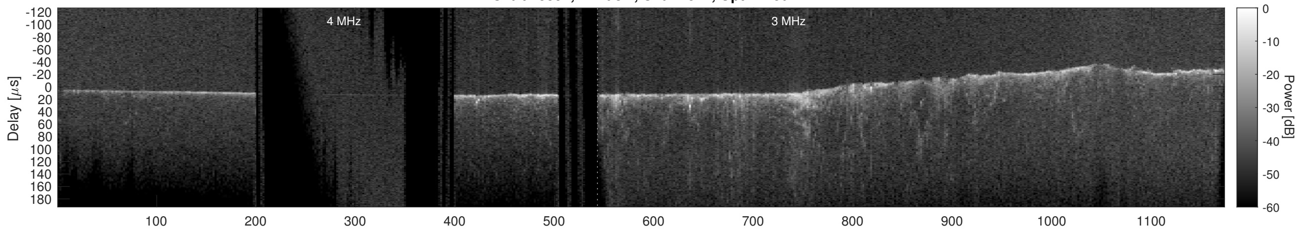
Orbit 15592, Cluttergram
