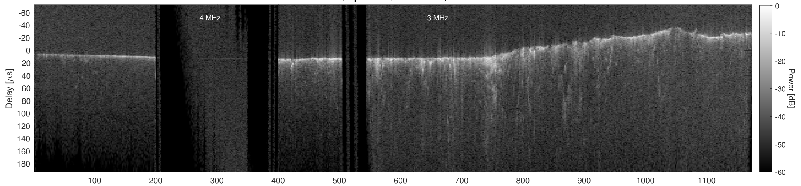
Orbit 15592, Cluttergram
