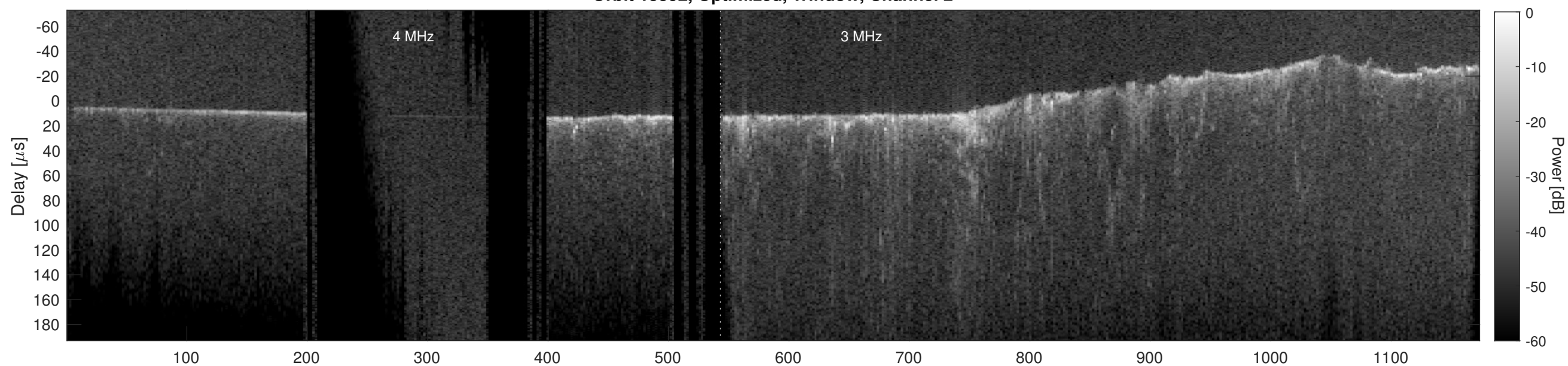
Orbit 15592, Cluttergram
