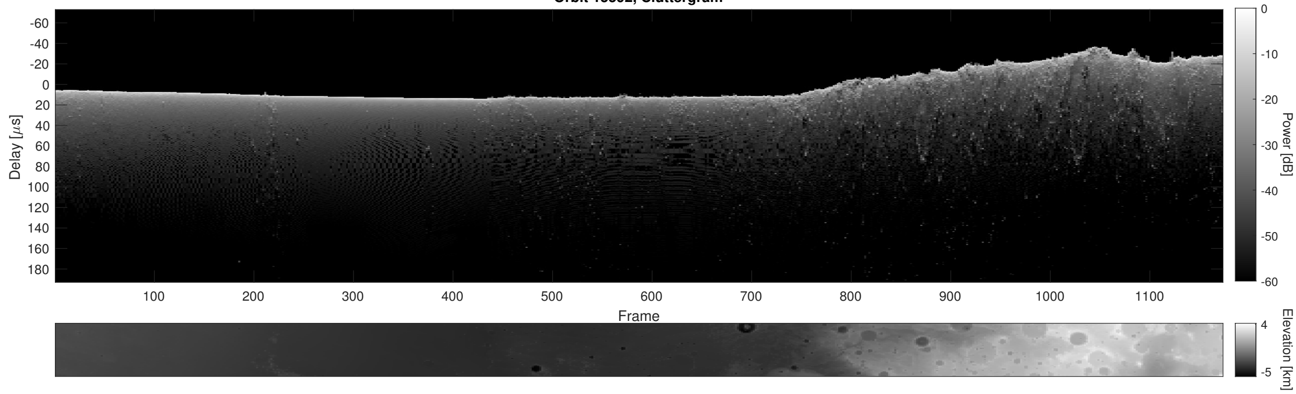
Orbit 15592, Cluttergram
