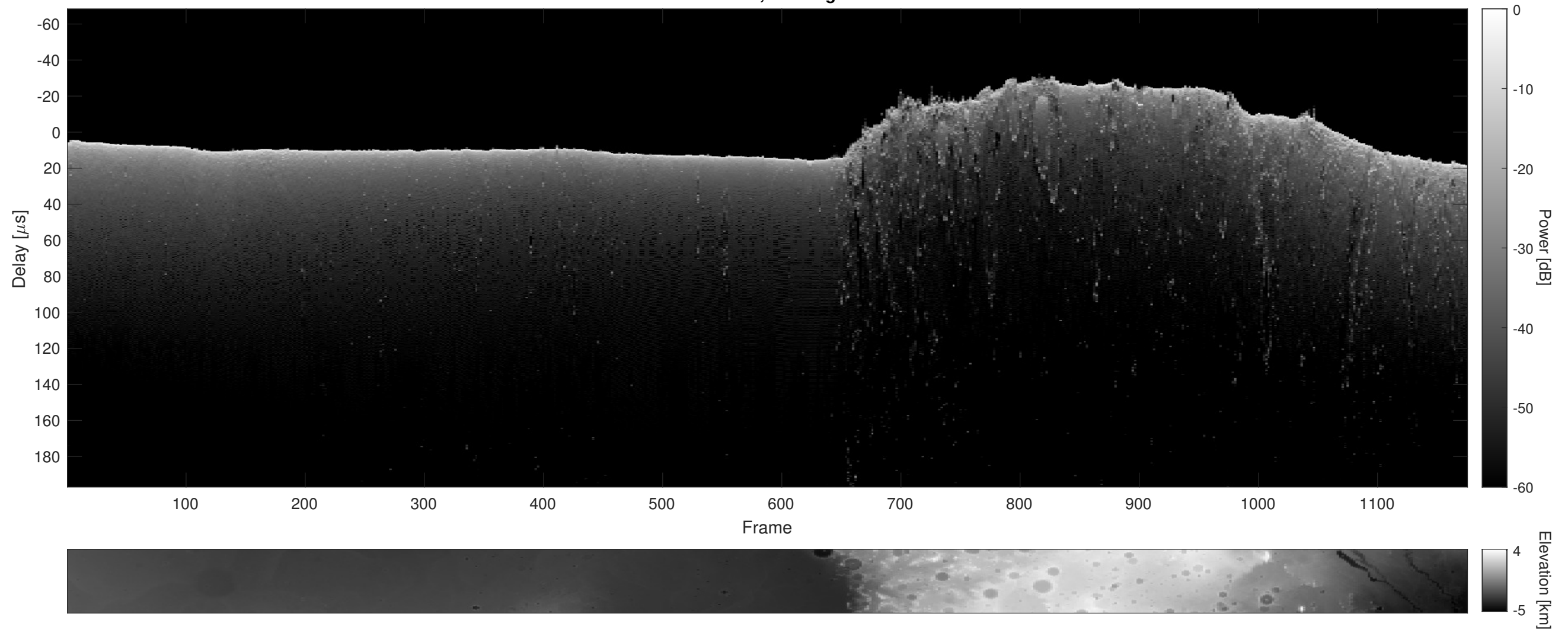
Orbit 15593, Cluttergram
