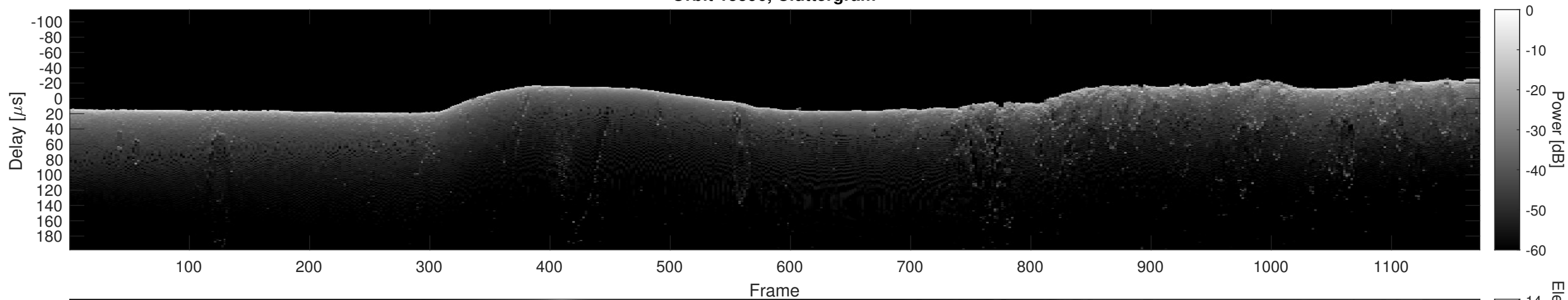
Orbit 15596, Cluttergram
