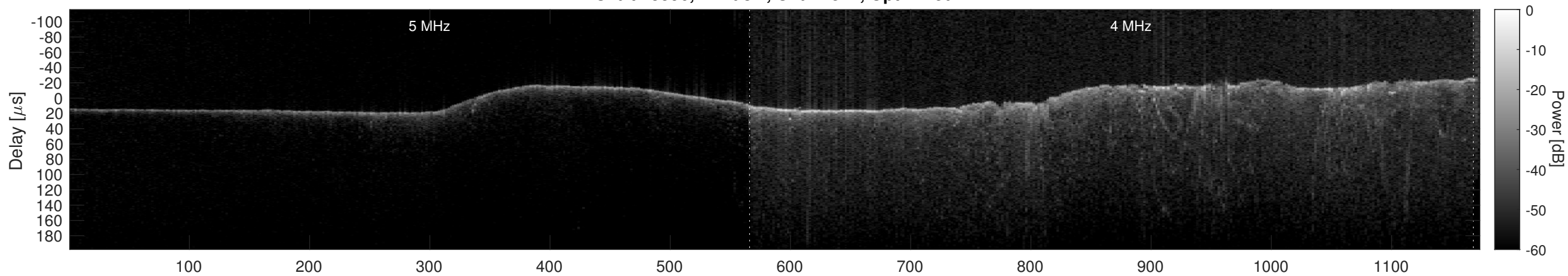
Orbit 15596, Cluttergram
