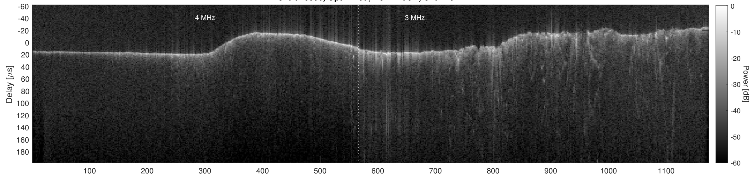
Orbit 15596, Cluttergram
