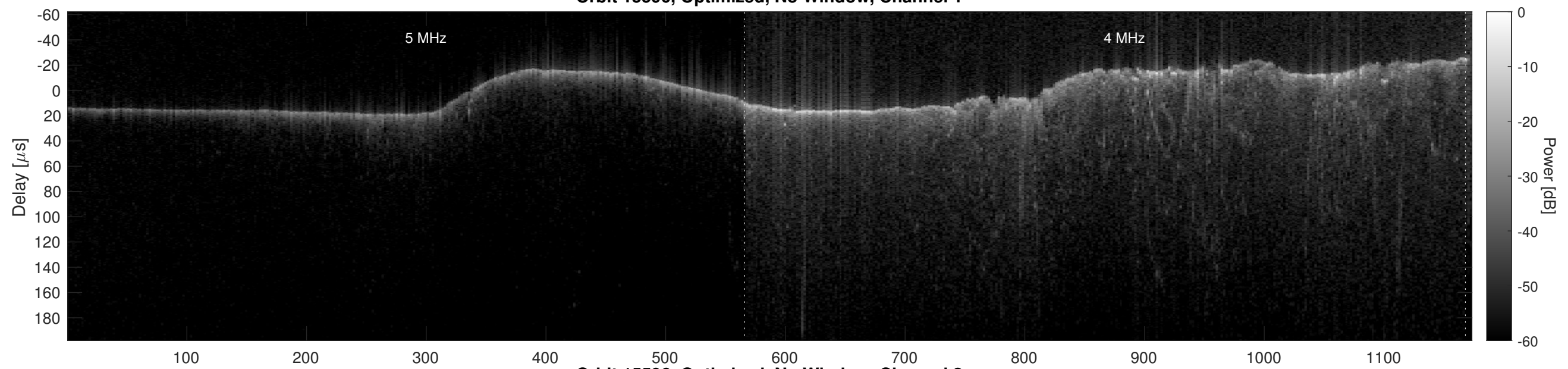
Orbit 15596, Optimized, No Window, Channel 2
