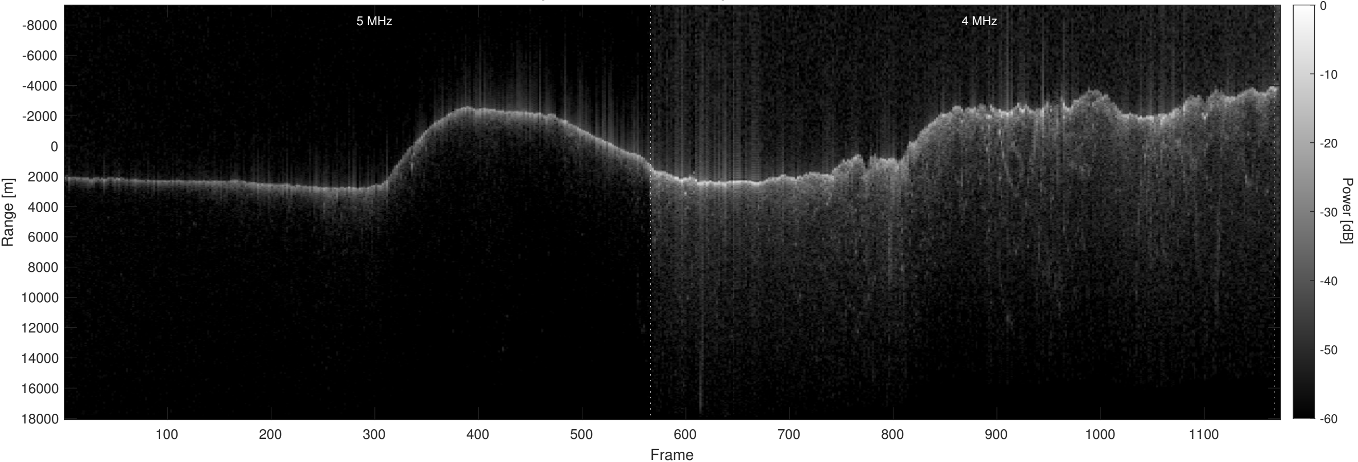
Orbit 15596, Optimized, No Window, Depth-Corrected, Channel 2
