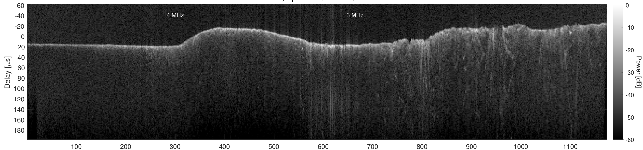
Orbit 15596, Cluttergram
