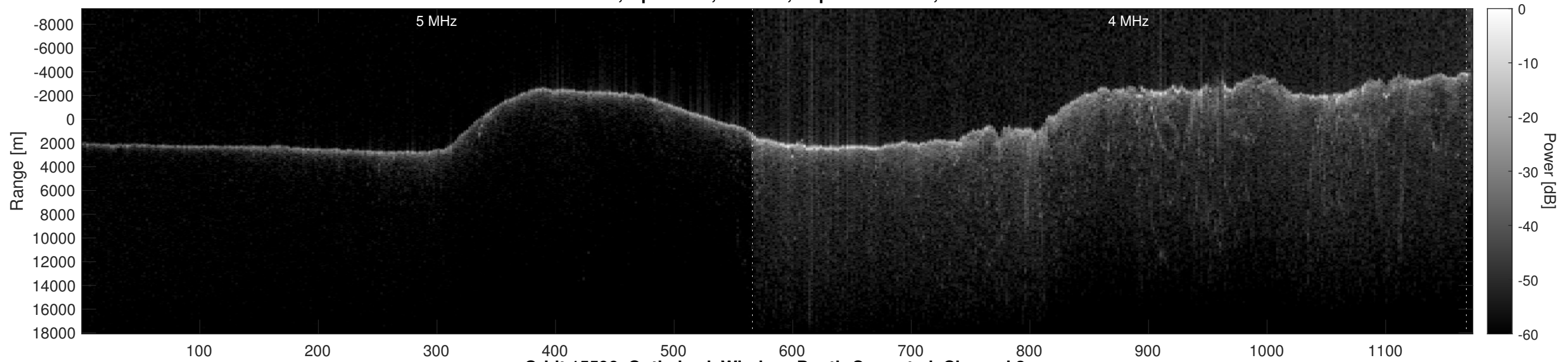
Orbit 15596, Optimized, Window, Depth-Corrected, Channel 2
