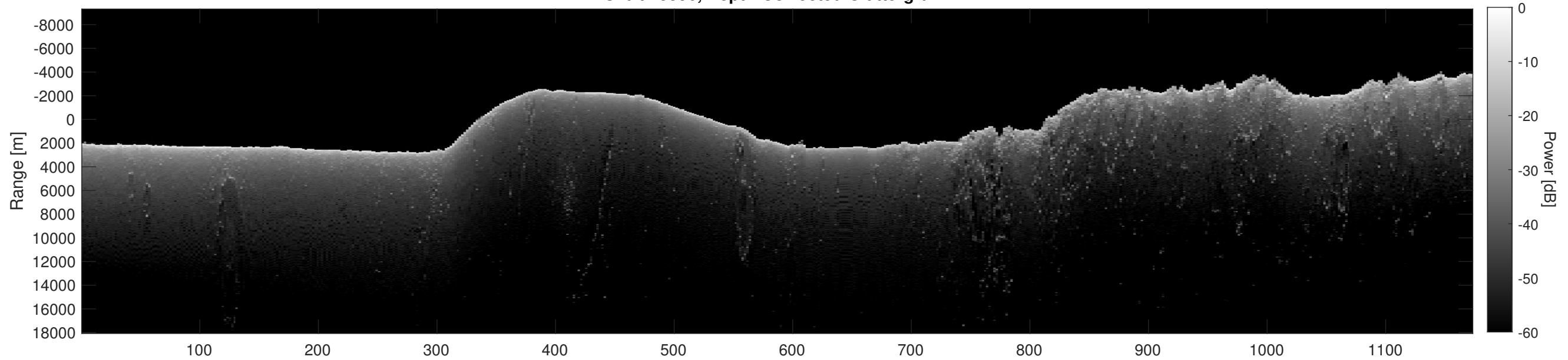
Orbit 15596, Depth-Corrected Cluttergram
