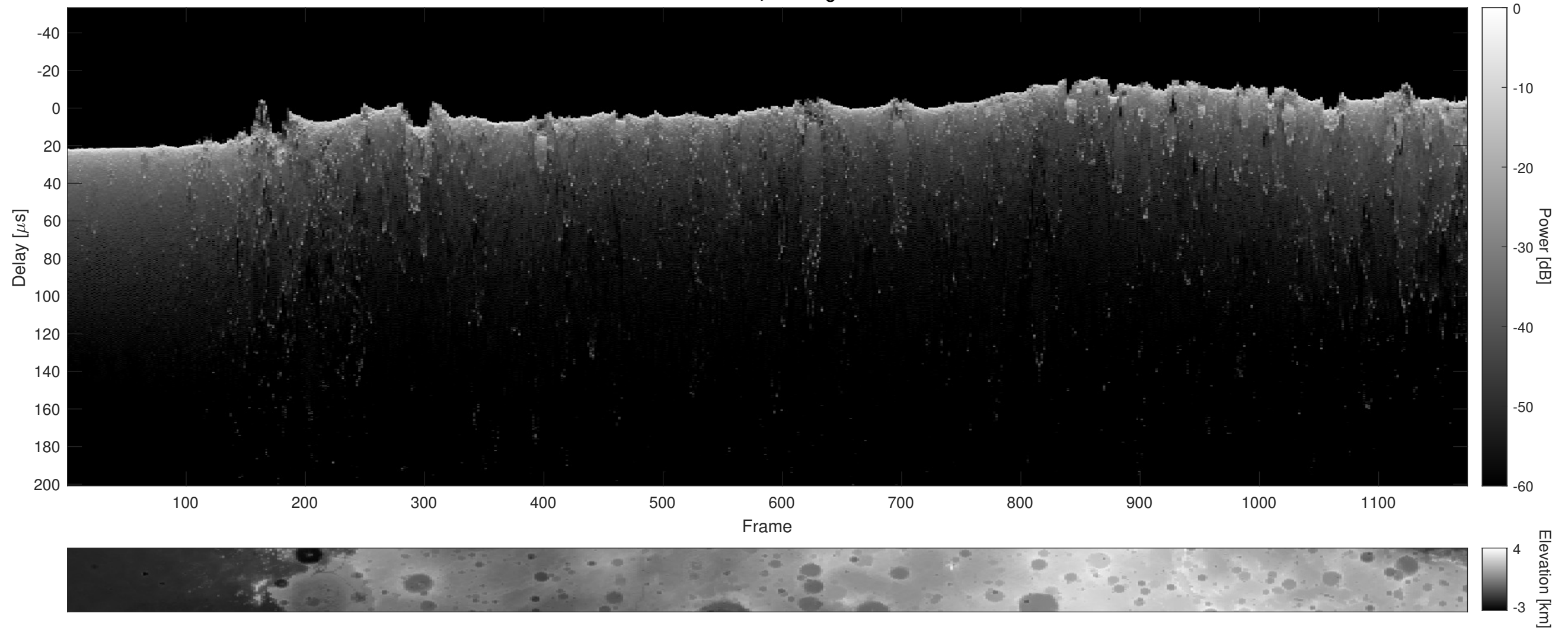
Orbit 15597, Cluttergram
