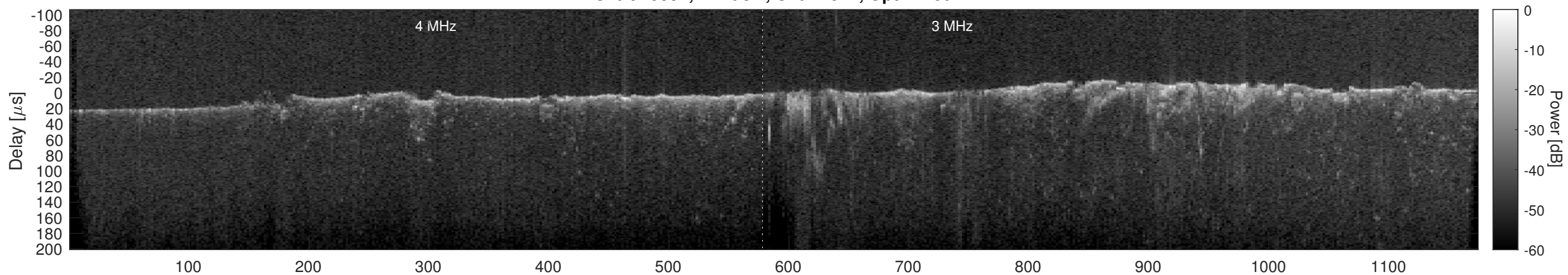
Orbit 15597, Cluttergram
