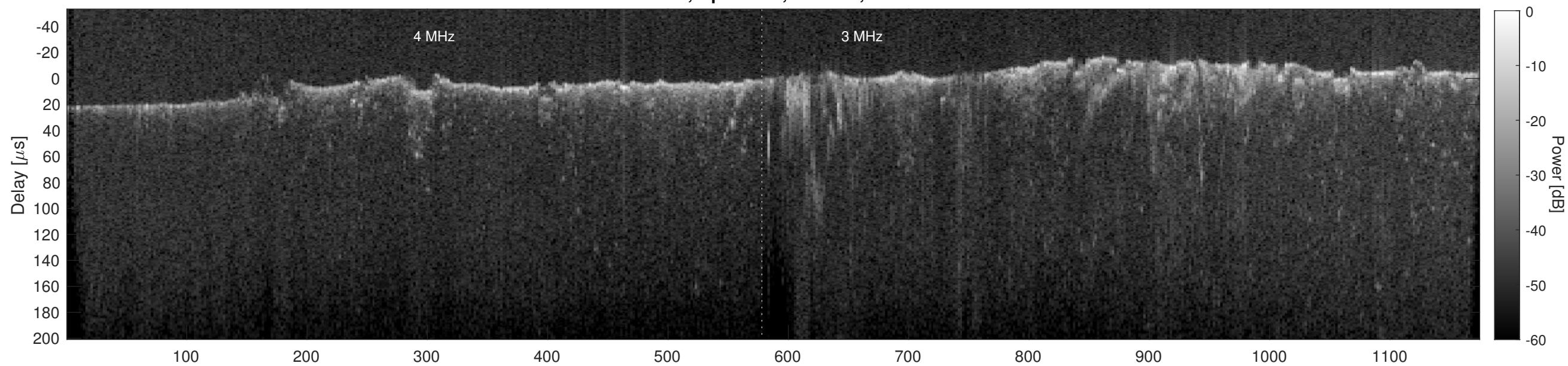
Orbit 15597, Cluttergram
