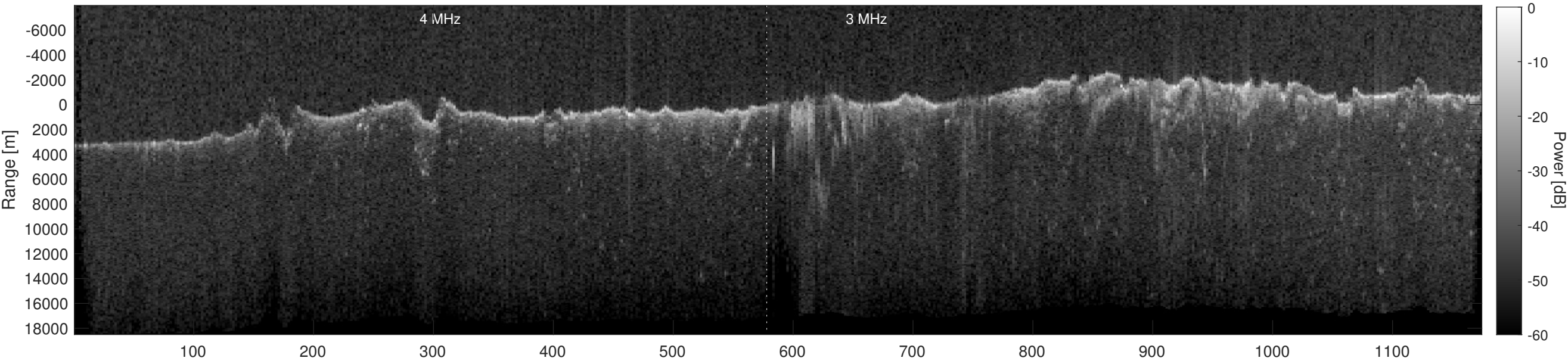
Orbit 15597, Depth-Corrected Cluttergram
