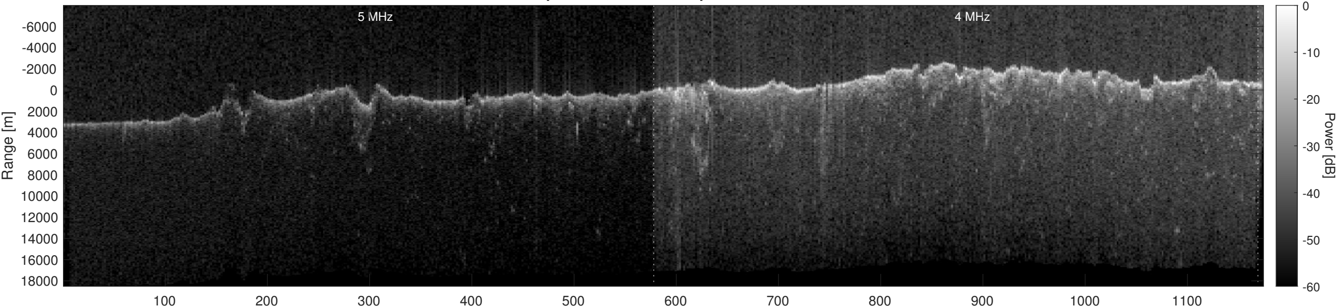
Orbit 15597, Optimized, Window, Depth-Corrected, Channel 2
