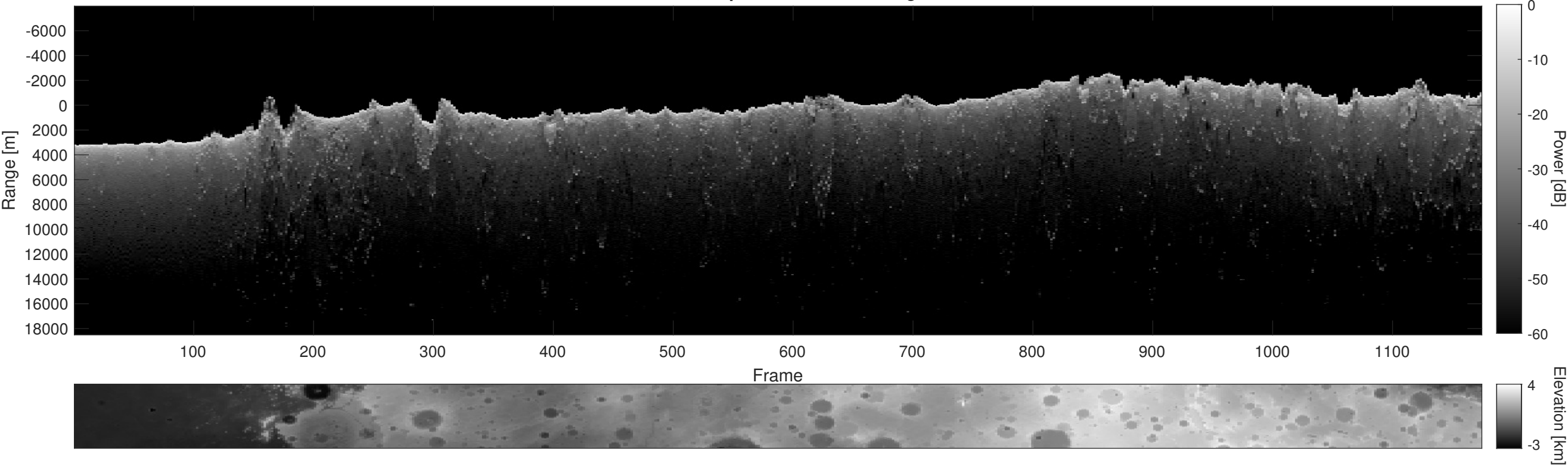
Orbit 15597, Depth-Corrected Cluttergram
