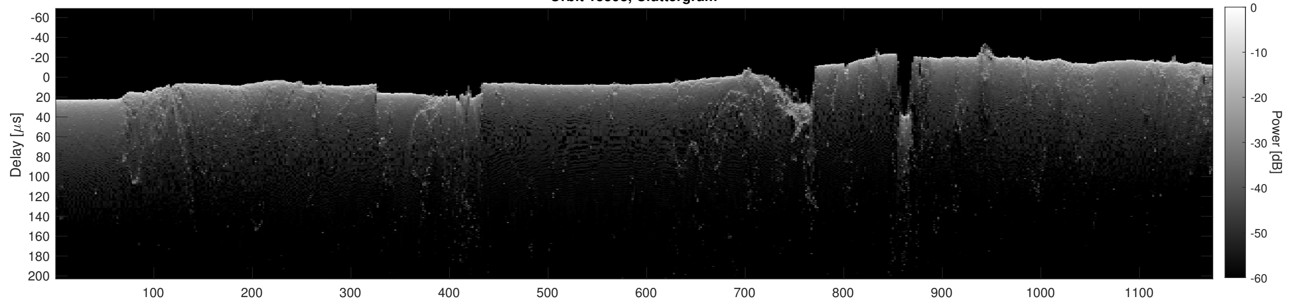
Orbit 15598, Cluttergram
