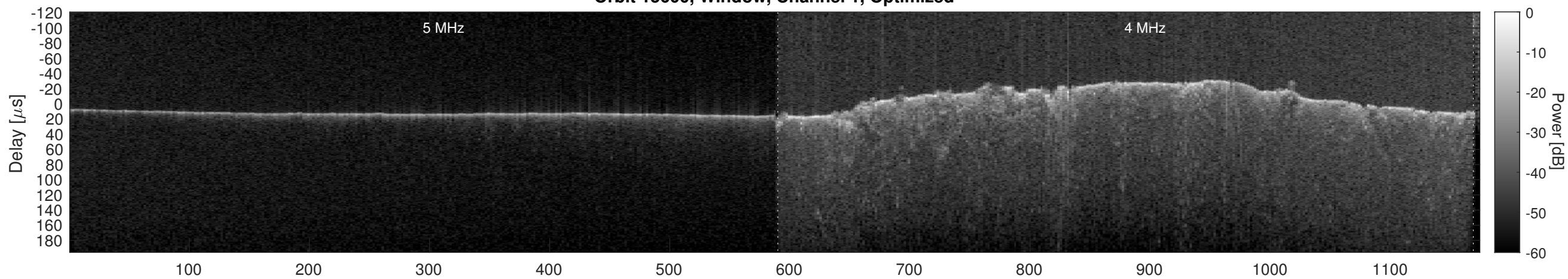
Orbit 15600, Cluttergram
