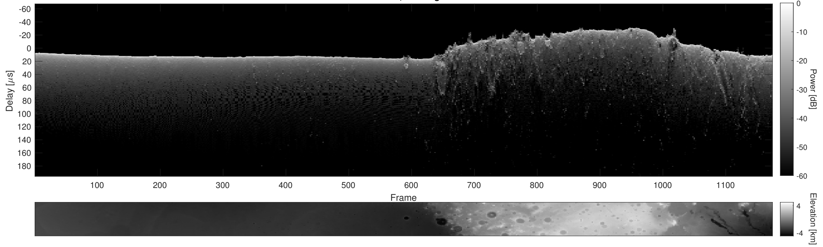
Orbit 15600, Cluttergram
