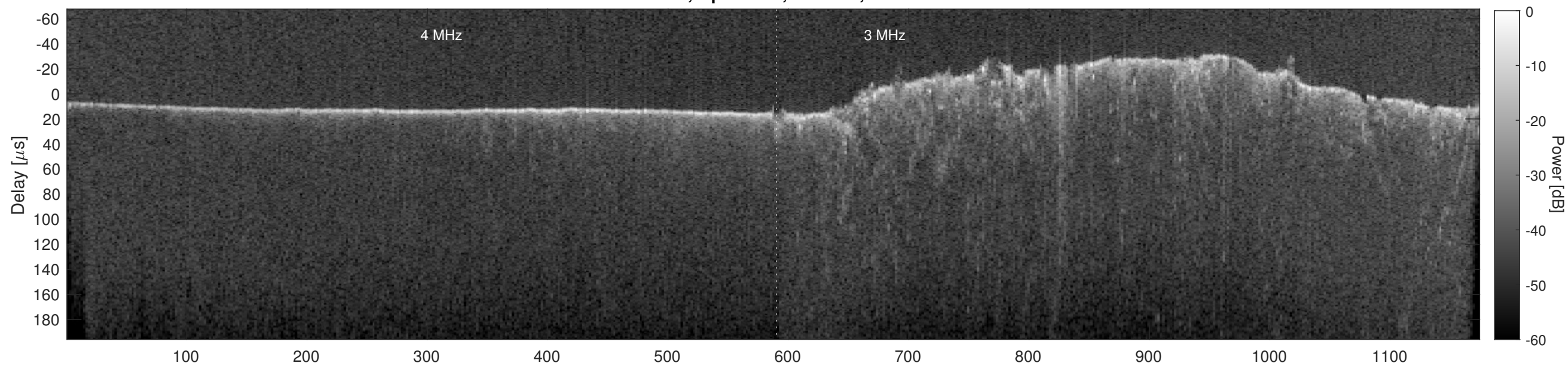
Orbit 15600, Cluttergram
