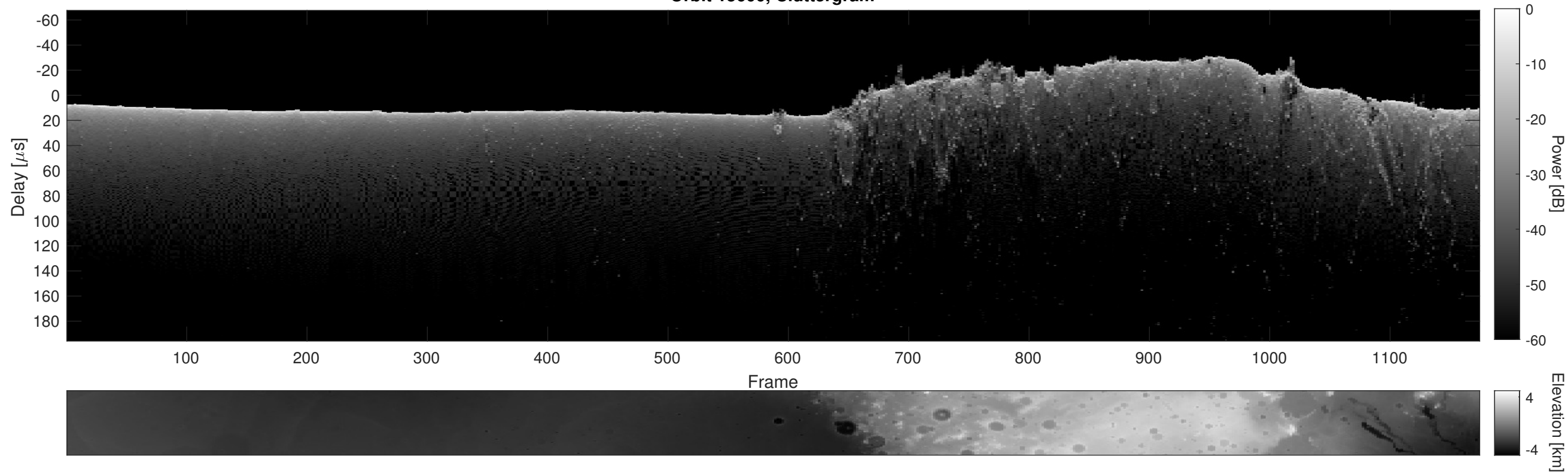
Orbit 15600, Cluttergram
