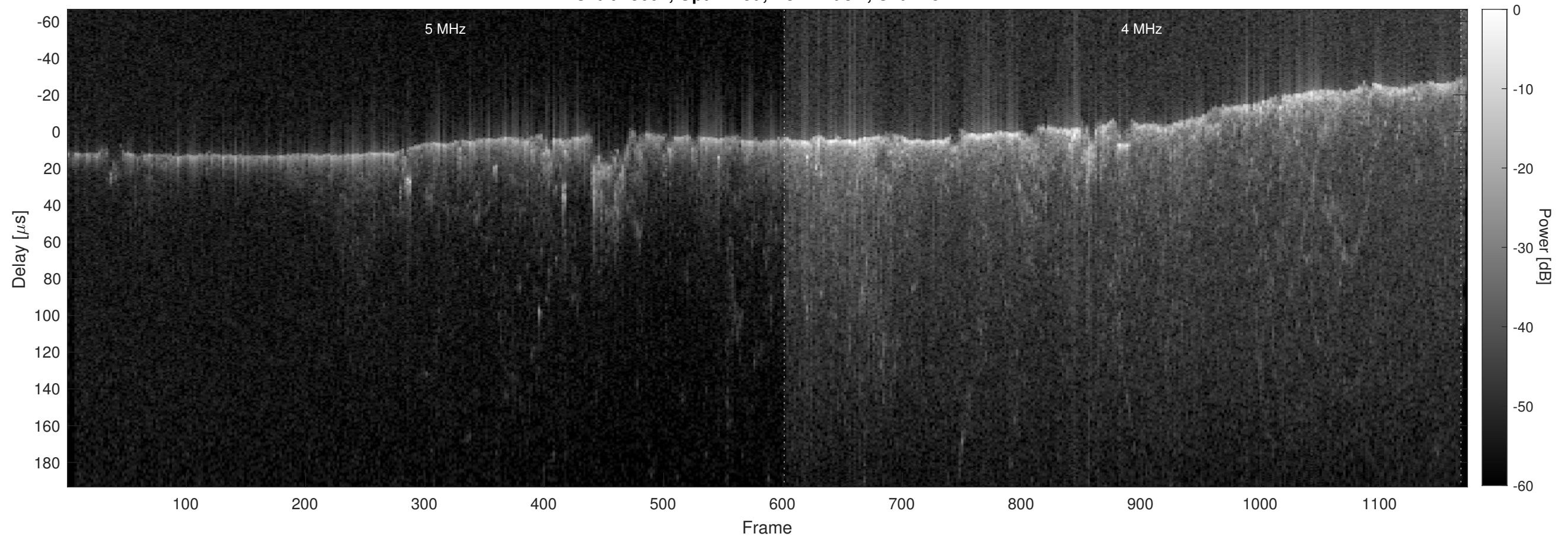
Orbit 15601, Optimized, No Window, Channel 2
