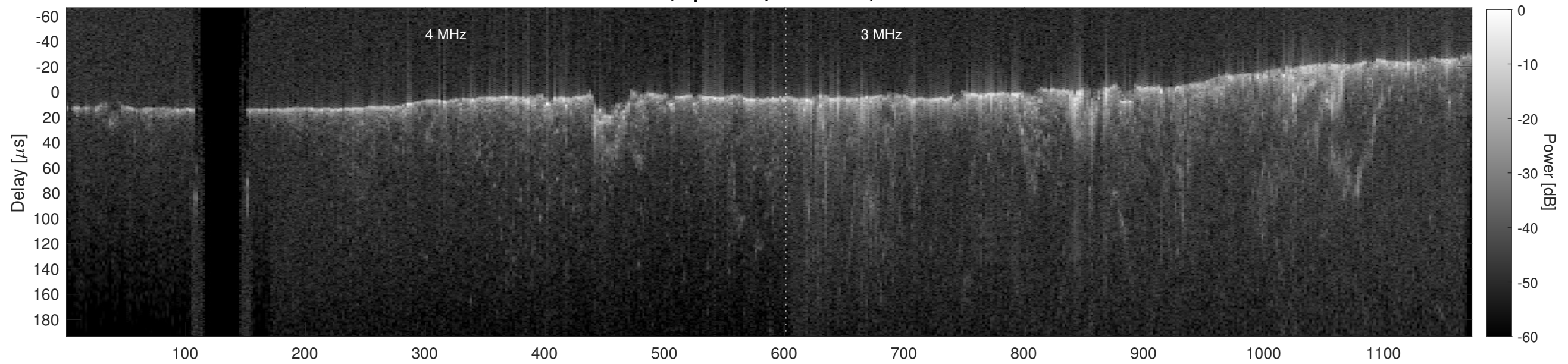
Orbit 15601, Cluttergram
