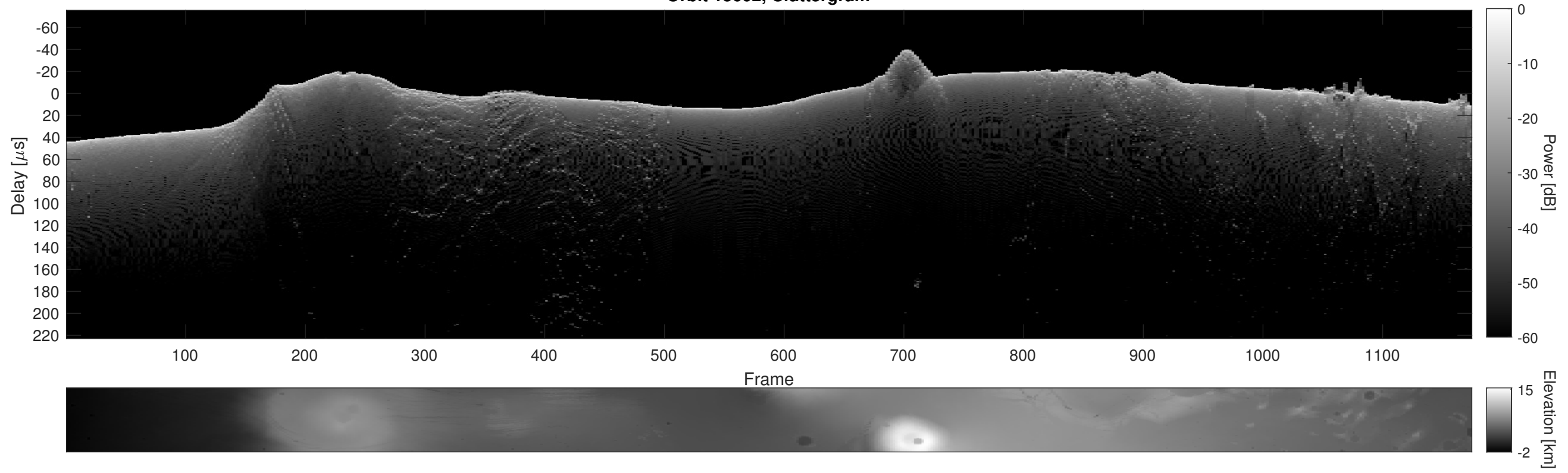
Orbit 15602, Cluttergram
