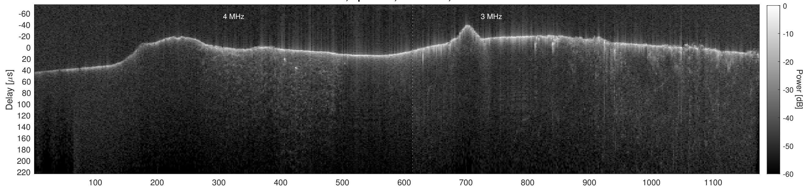
Orbit 15602, Cluttergram
