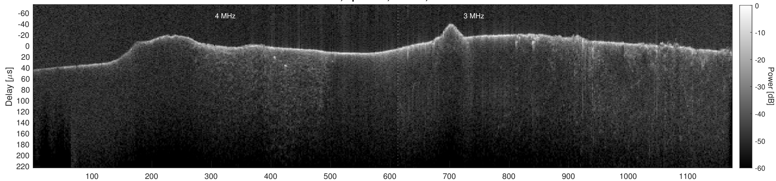
Orbit 15602, Cluttergram
