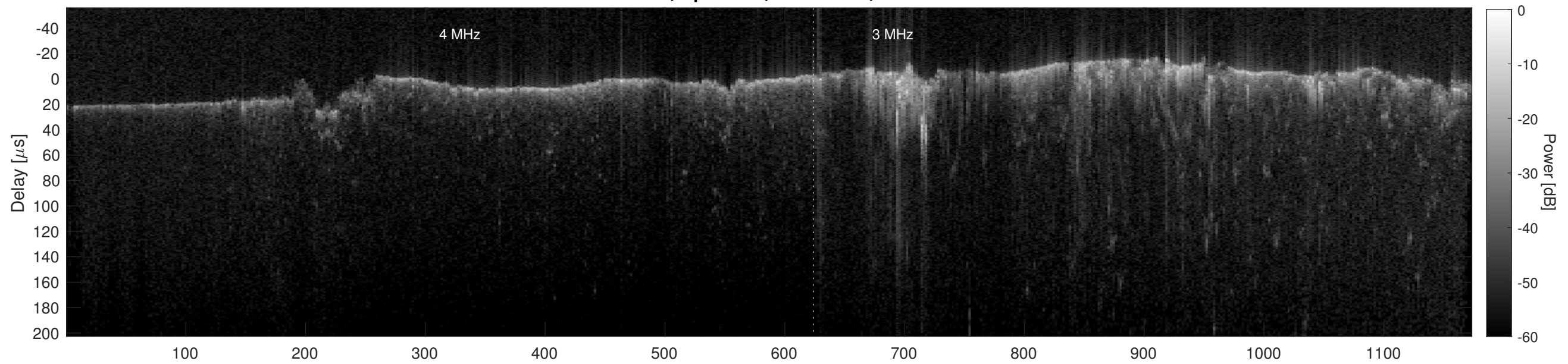
Orbit 15604, Cluttergram
