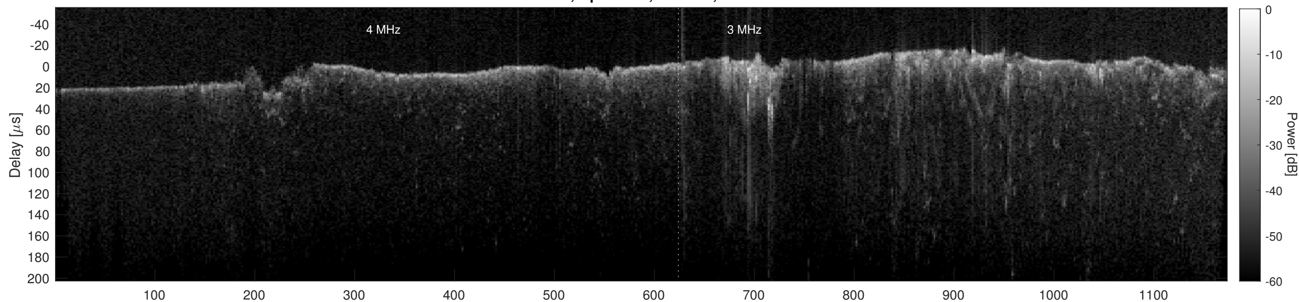
Orbit 15604, Cluttergram
