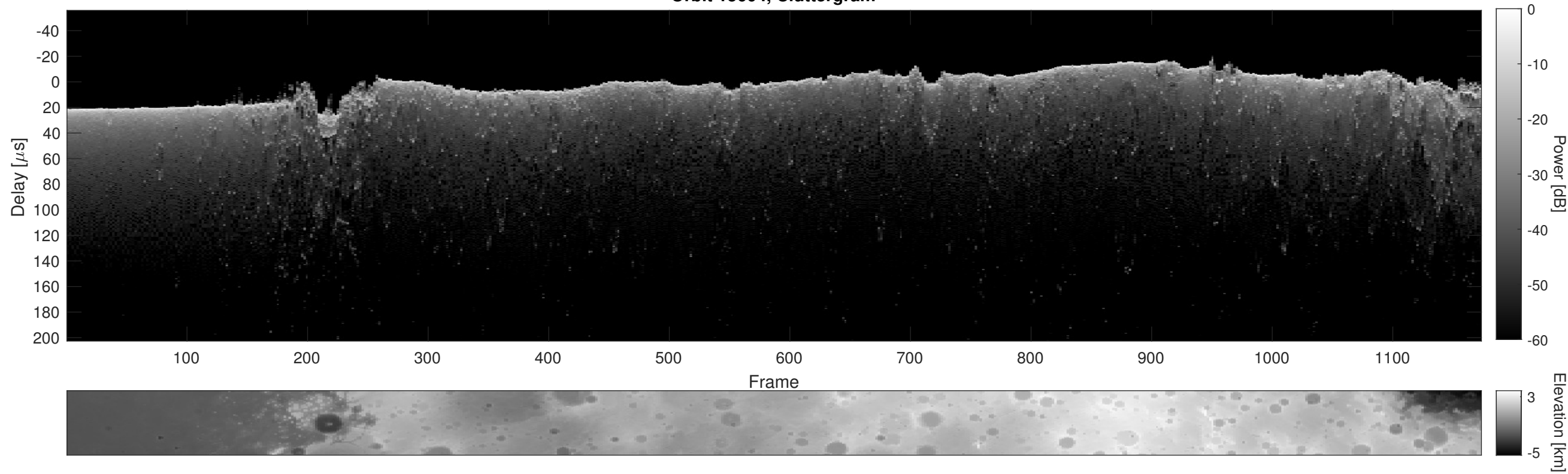
Orbit 15604, Cluttergram
