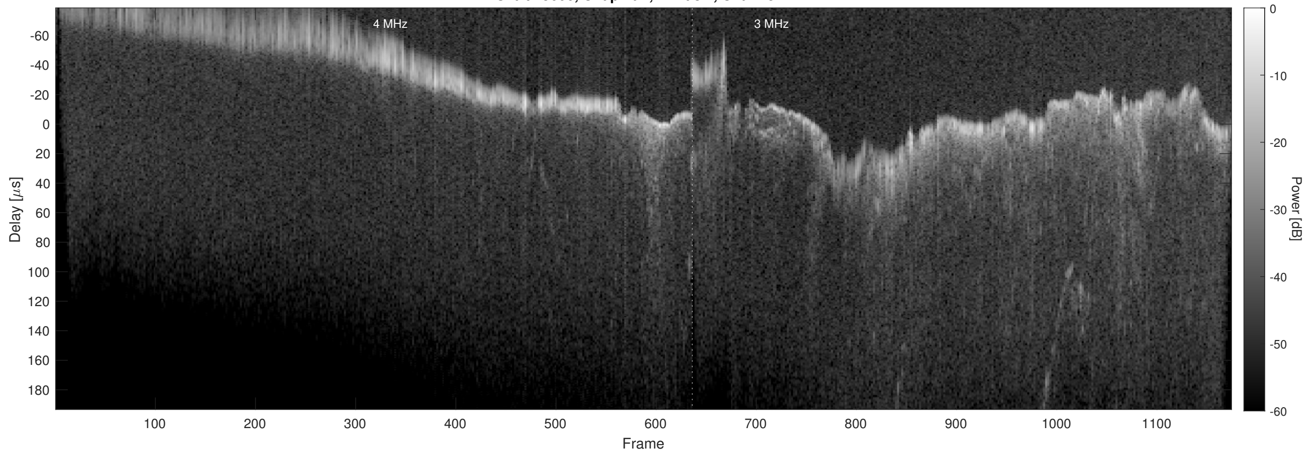
Orbit 15606, Chapman, Window, Channel 2
