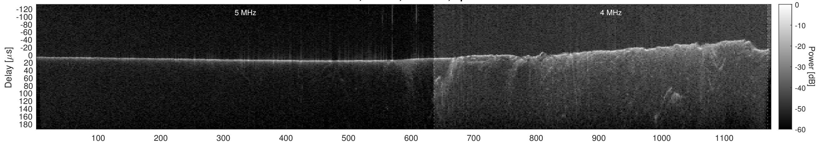
Orbit 15606, Cluttergram
