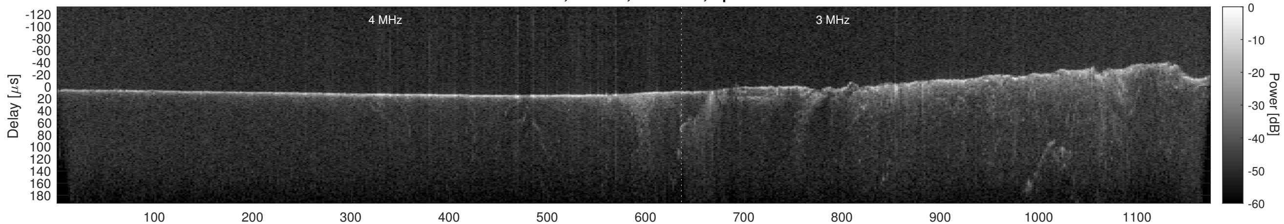
Orbit 15606, Cluttergram
