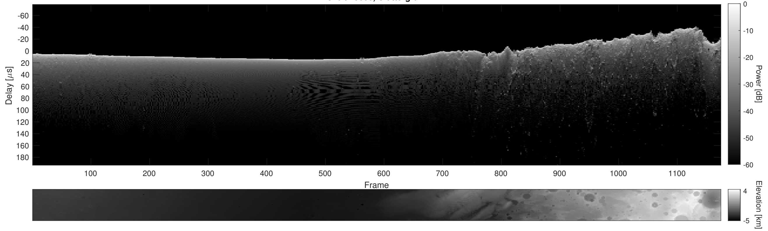
Orbit 15606, Cluttergram
