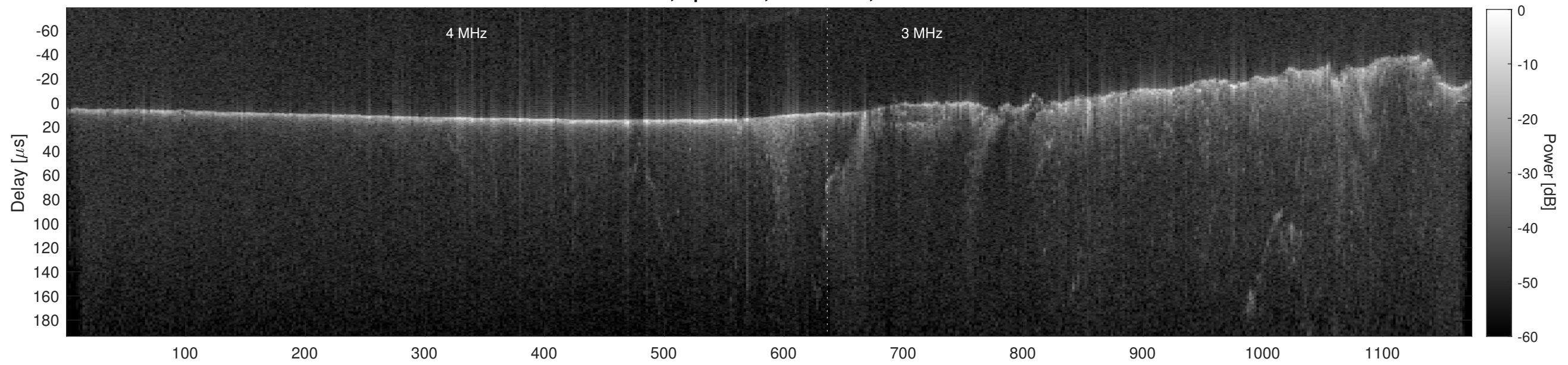
Orbit 15606, Cluttergram
