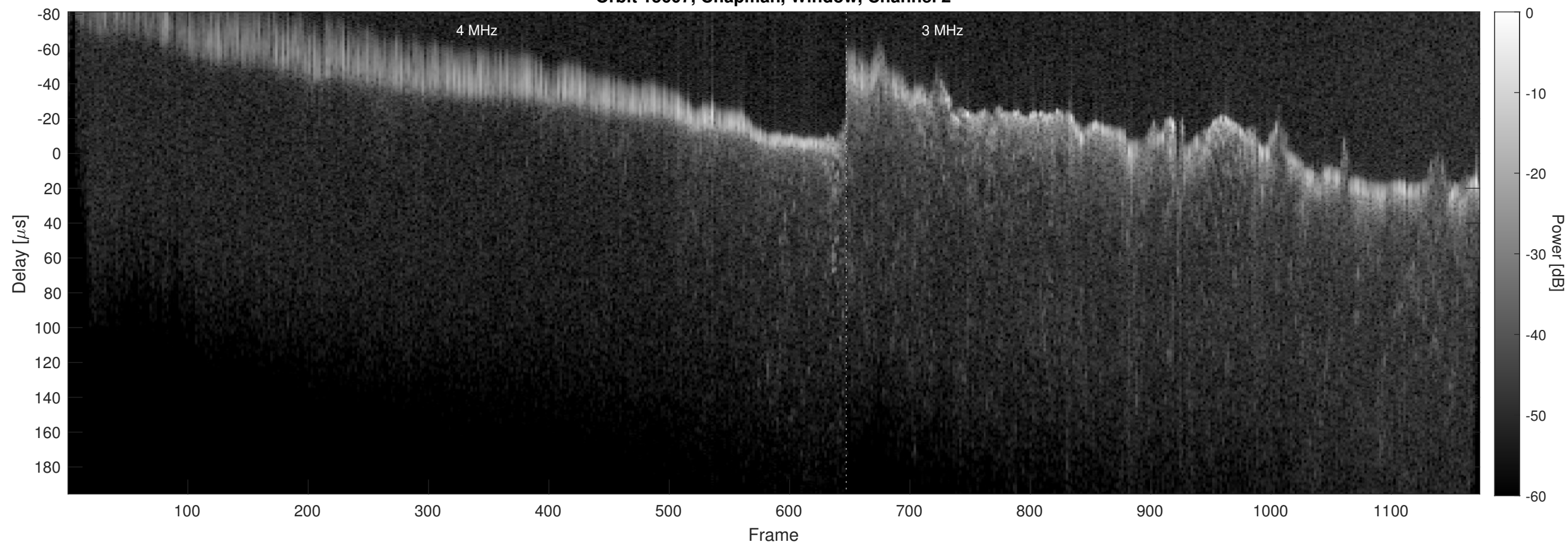
Orbit 15607, Chapman, Window, Channel 2
