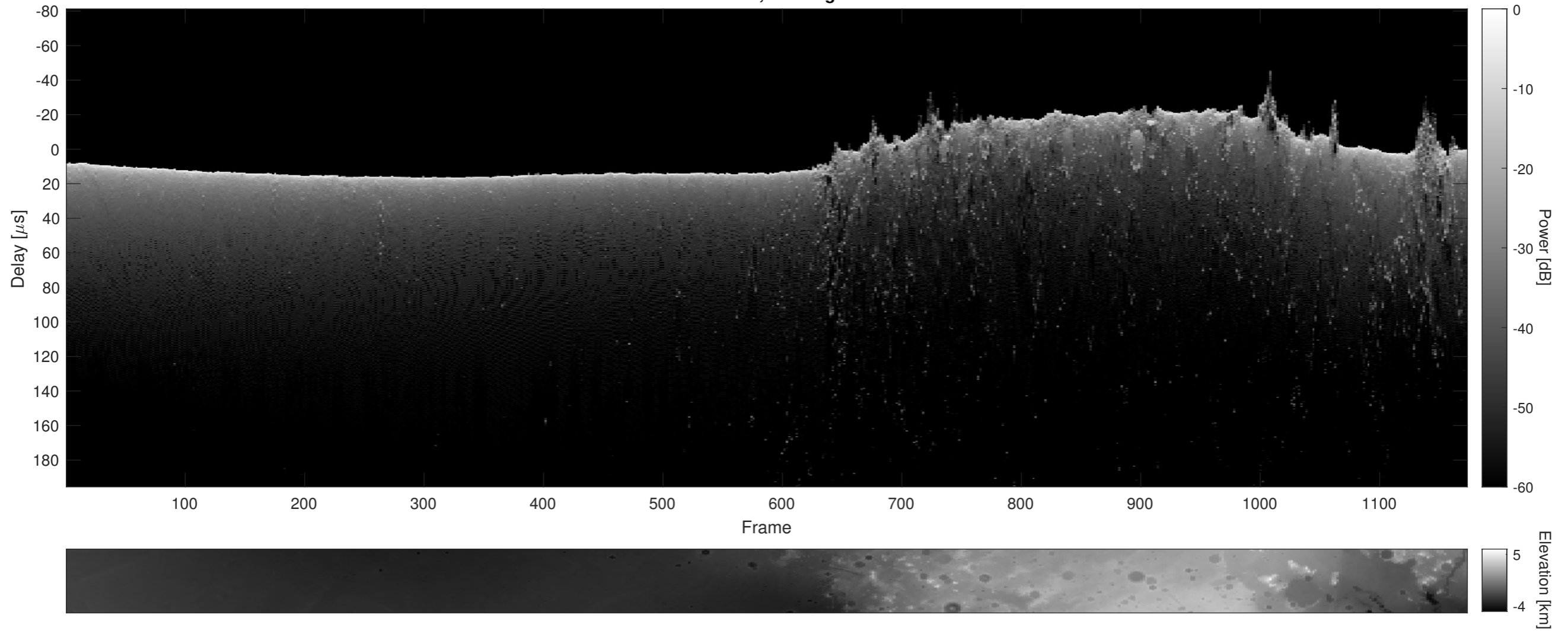
Orbit 15607, Cluttergram
