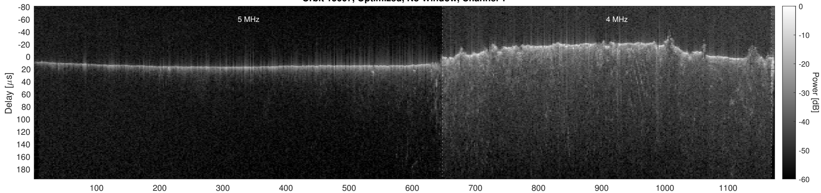
Orbit 15607, Optimized, No Window, Channel 2
