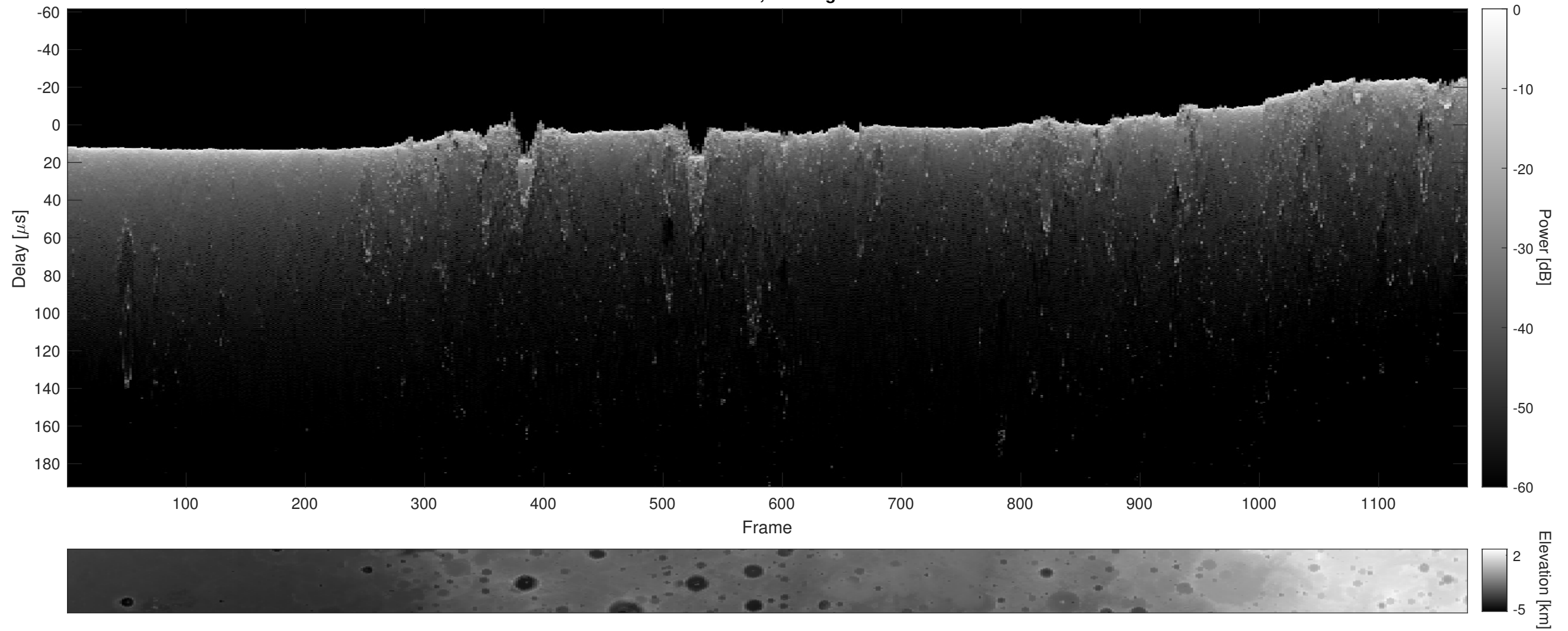
Orbit 15608, Cluttergram
