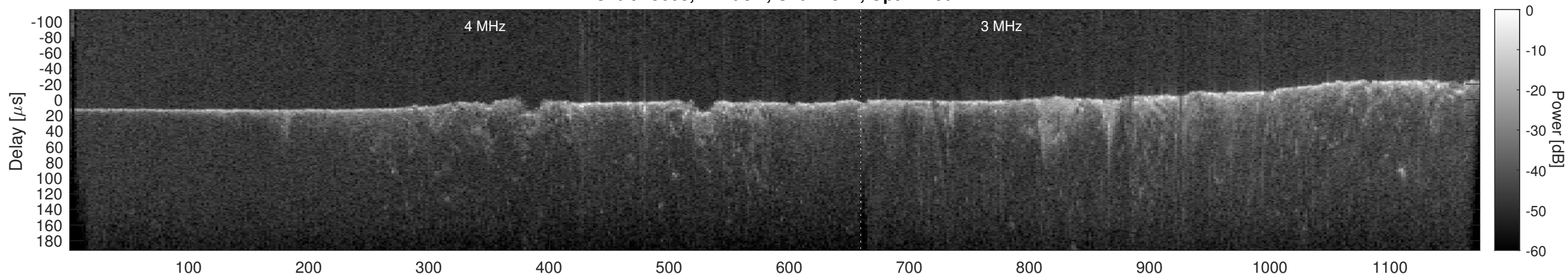
Orbit 15608, Cluttergram
