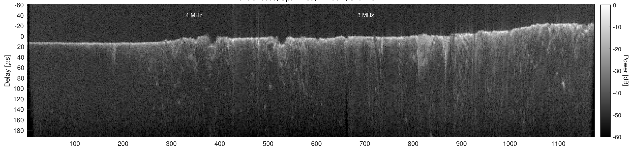
Orbit 15608, Cluttergram
