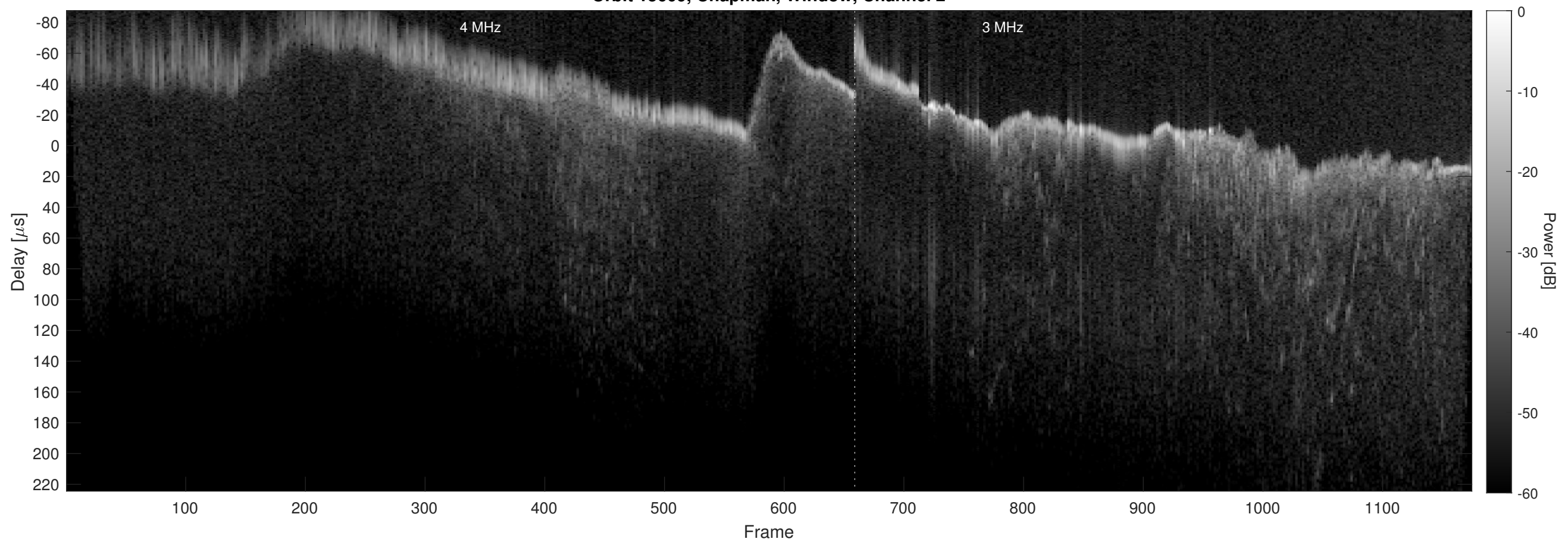
Orbit 15609, Chapman, Window, Channel 2
