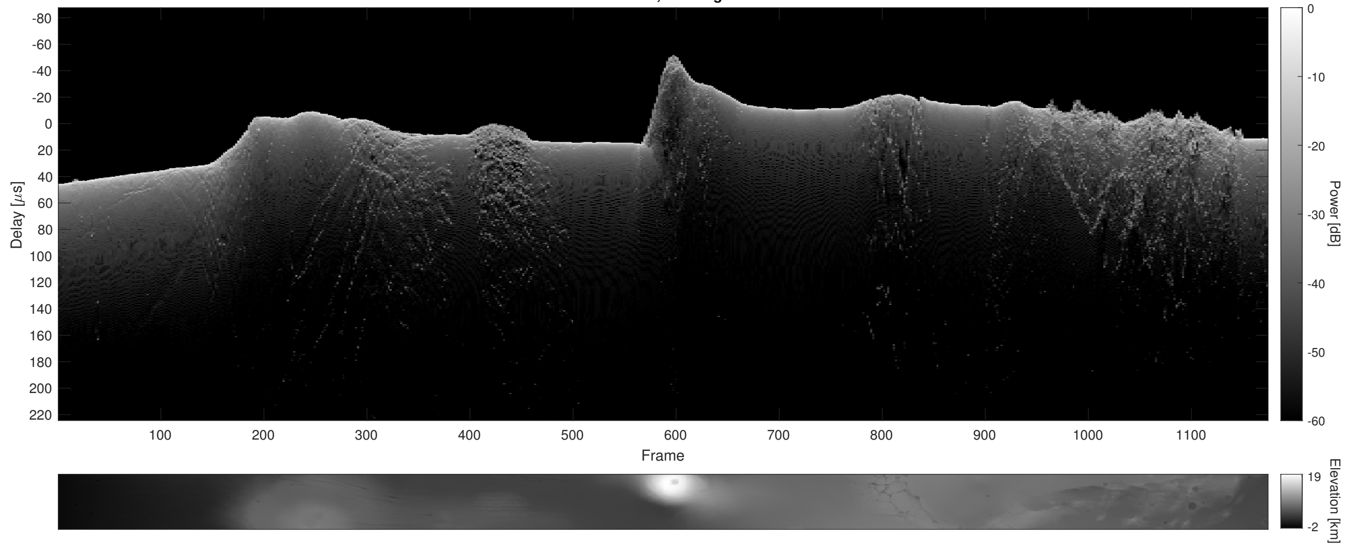
Orbit 15609, Cluttergram
