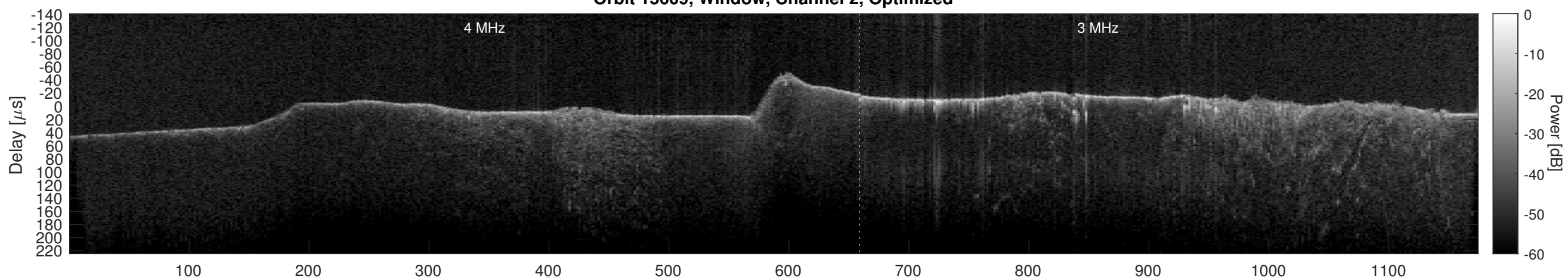
Orbit 15609, Cluttergram
