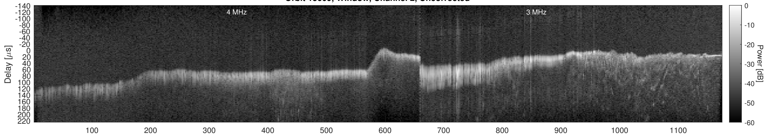
Orbit 15609, Window, Channel 2, Chapman
