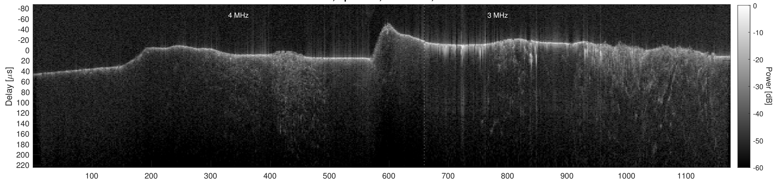
Orbit 15609, Cluttergram
