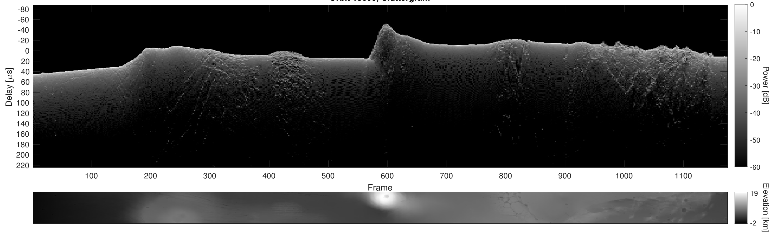
Orbit 15609, Cluttergram
