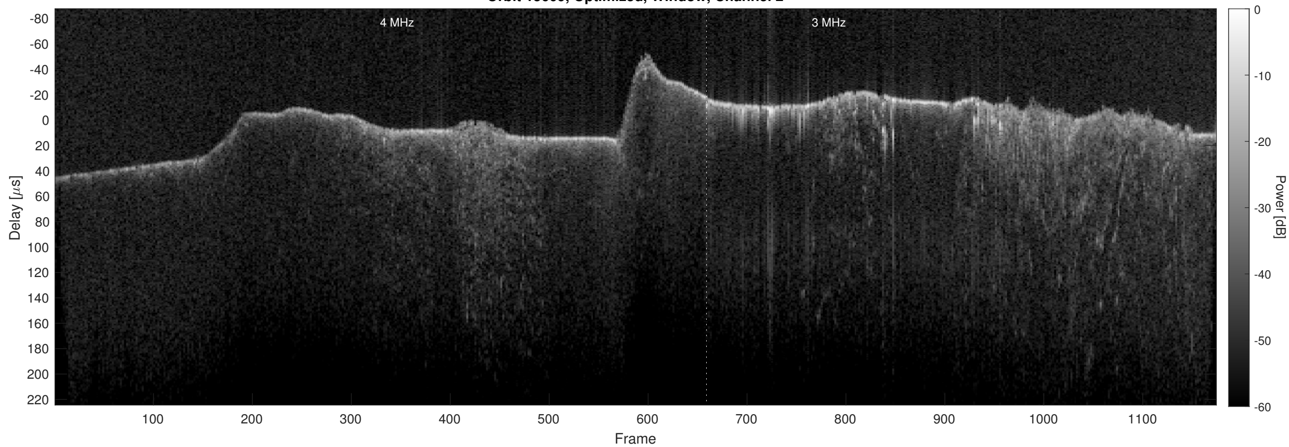
Orbit 15609, Optimized, Window, Channel 2
