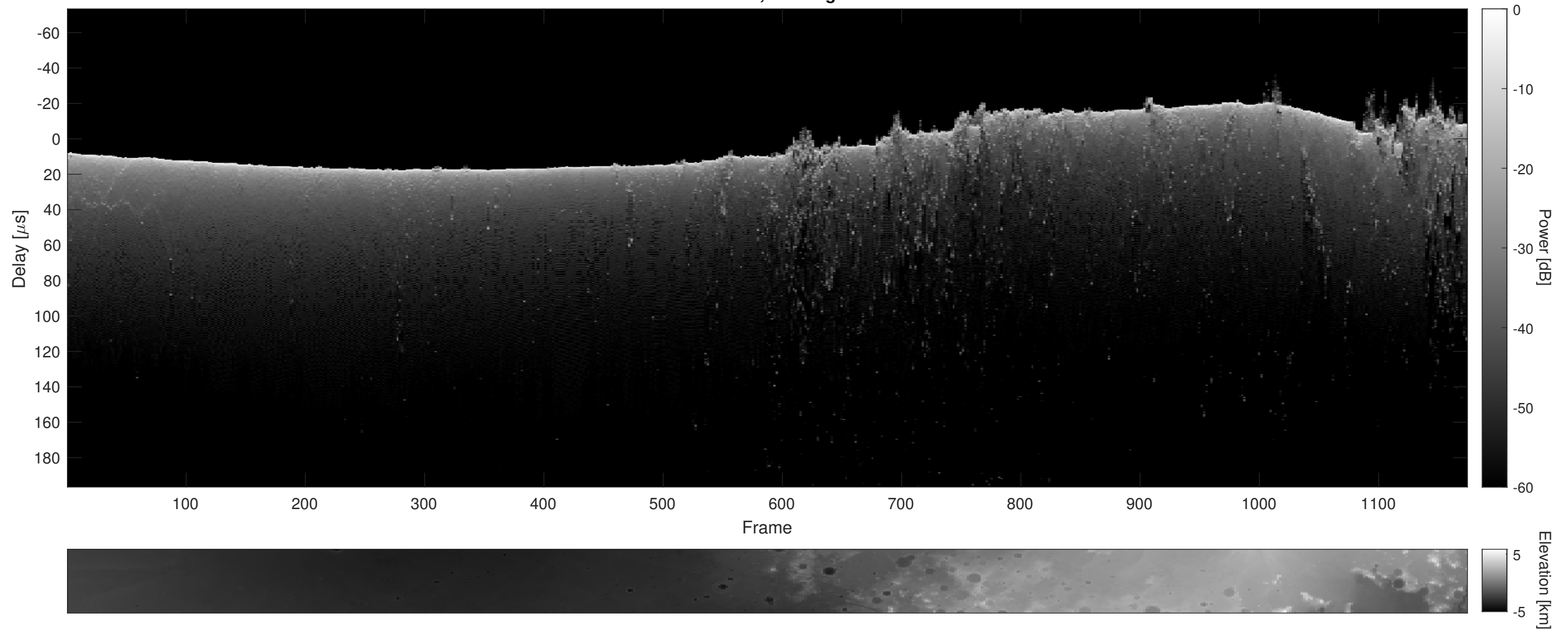
Orbit 15614, Cluttergram
