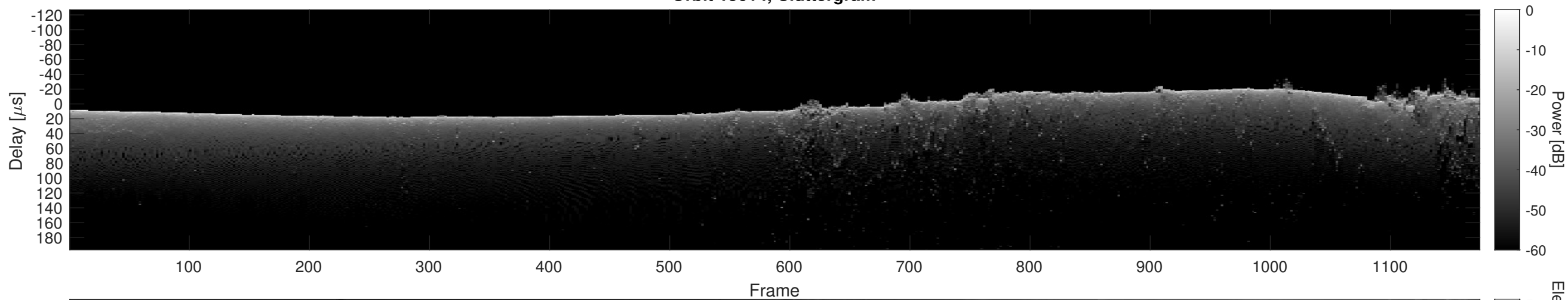
Orbit 15614, Cluttergram
